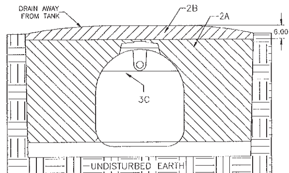
Figure 3: Backfilling
