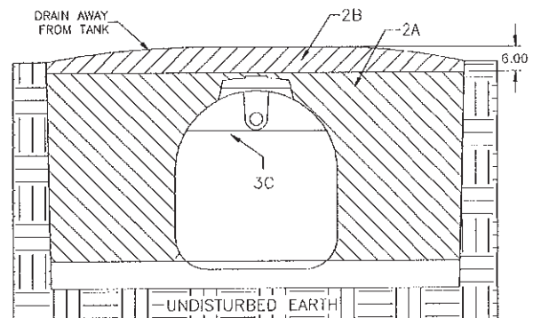
Figure 3: Backfilling
