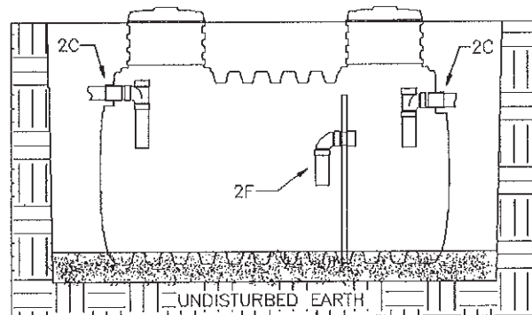
Figure 2: Tank Assembly / Installation
